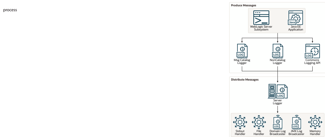
Figure 1-1 WebLogic Server Logging Process
