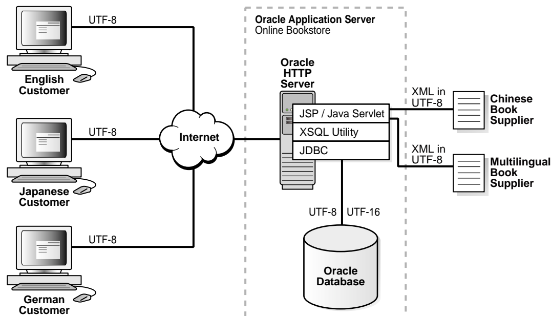
Figure 7-1 World-of-Books Architecture
